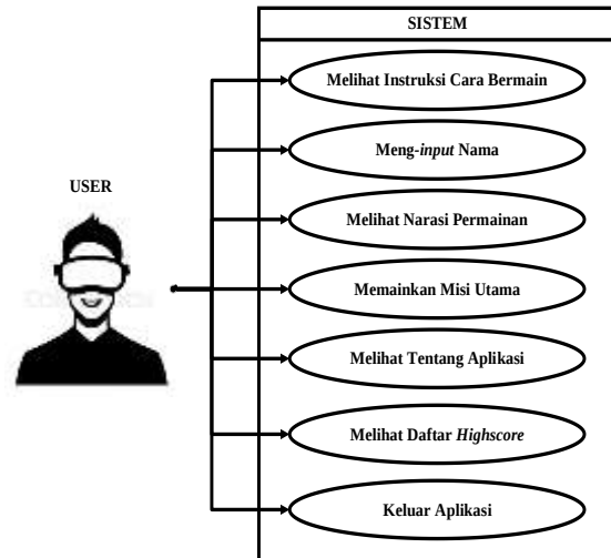
Gambar 4. Use Case
