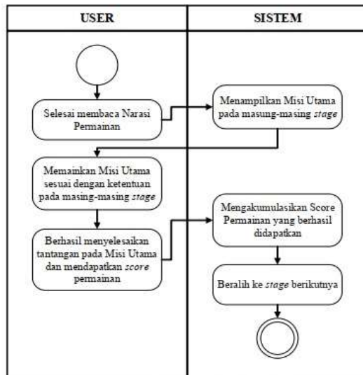
Gambar 5. Activity Diagram
