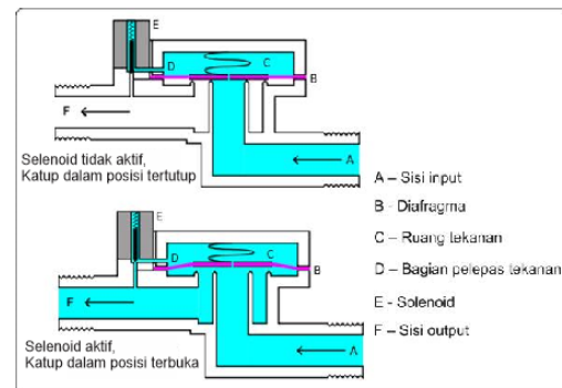
Gambar 4. Prinsip Kerja Selenoid Valve
