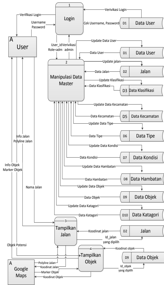
Gambar 3 DFD Level 0
