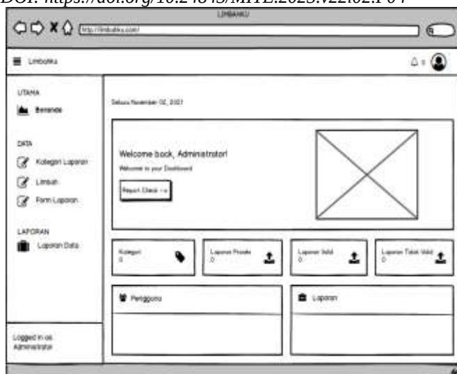
Gambar 7: Desain Halaman Dashboard Admin
