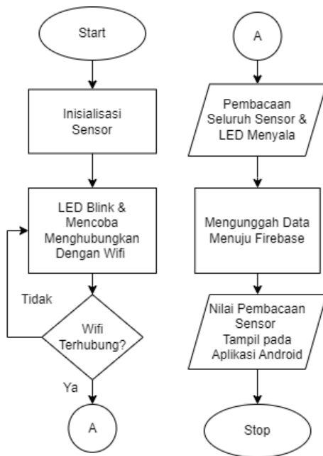
Gambar 4: Diagram Alir Program
