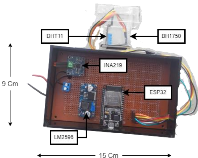
Gambar 8: Hardware Sistem
