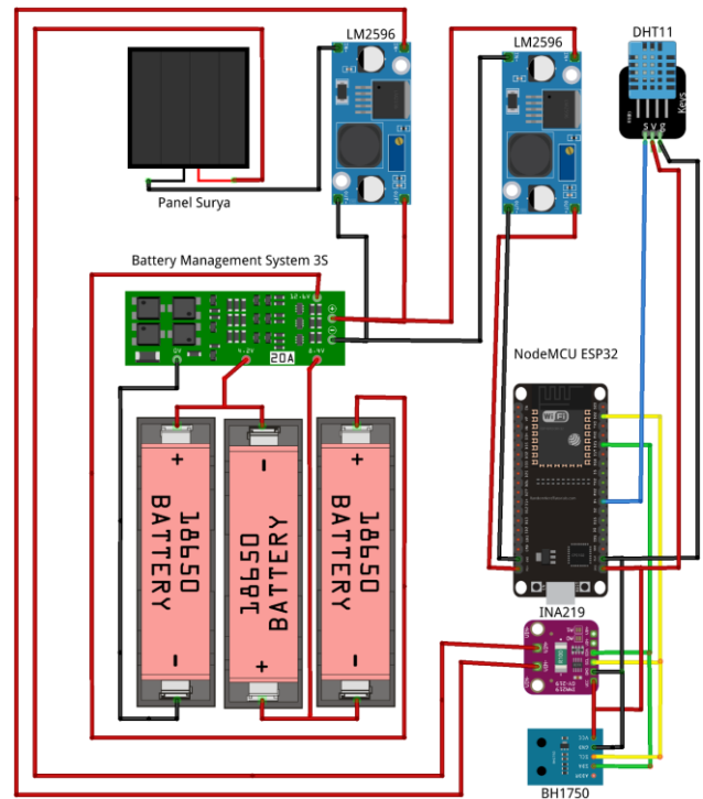
Gambar 3: Wiring Diagram sistem
