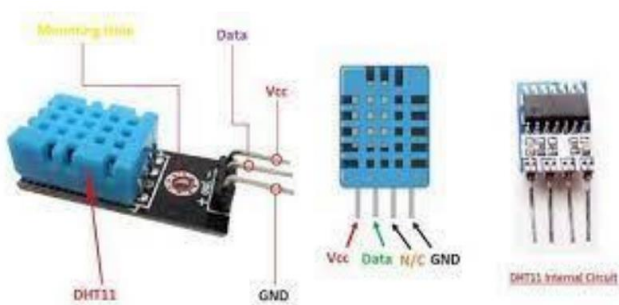
Gambar 4. Sensor Suhu
