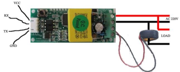
Gambar 5. Sensor Arus
