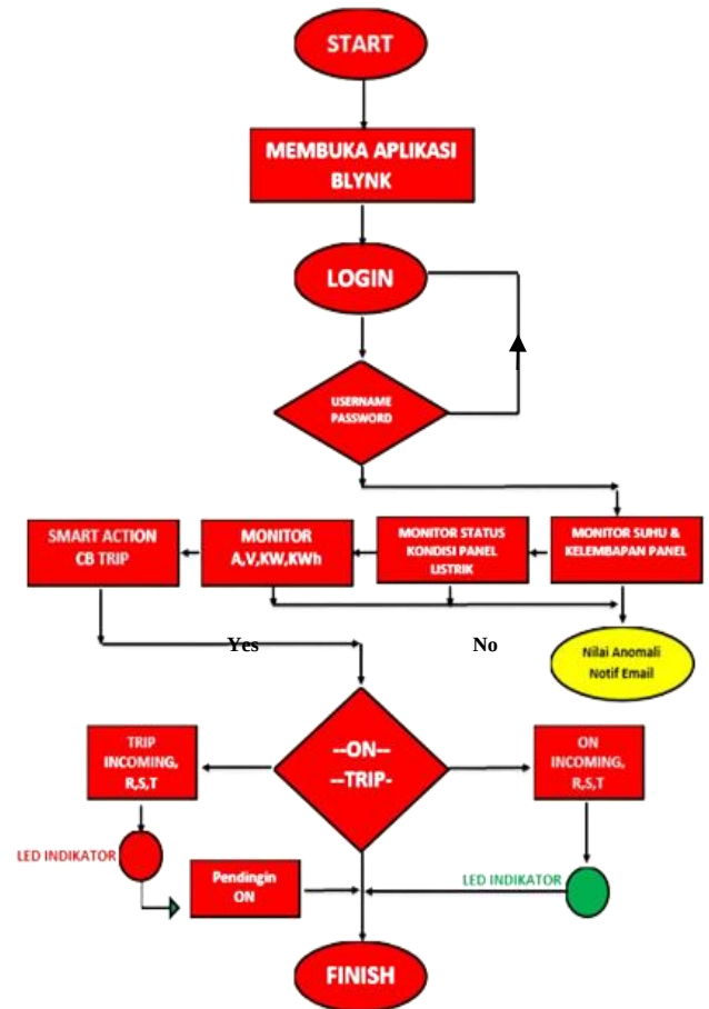
Gambar 9. Flowchart System
