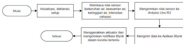
Gambar 3: Alur Sistem IoT
