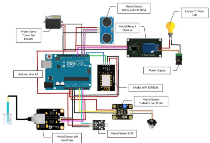
Gambar 5: Perancangan Rangkaian Hardware
