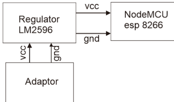
Gambar 6: diagram blok regulator LM 2596
