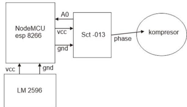
Gambar 7: Diagram Blok Pengujian Sensor Sct-013.
