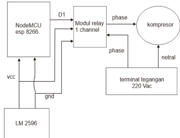
Gambar 10: Diagram blok modul relay 1 channel
