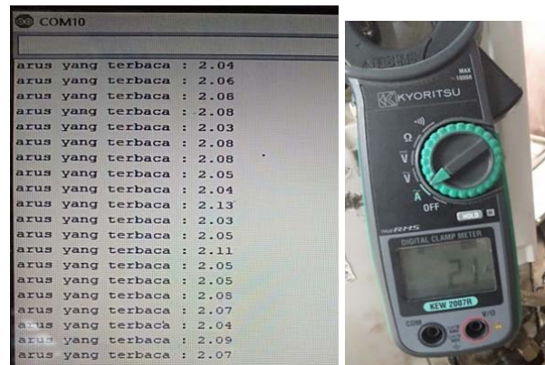
Gambar 22: Pengujian Sensor Arus Sct-013
