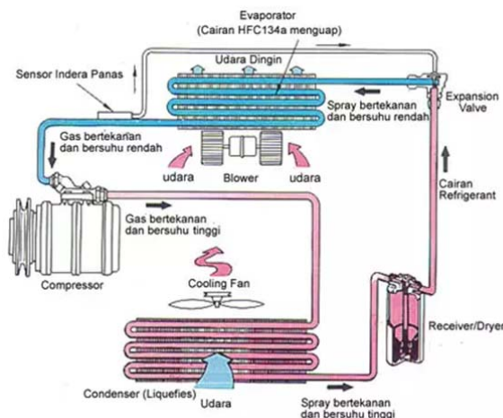
Gambar 1: cara kerja Air Conditioner
