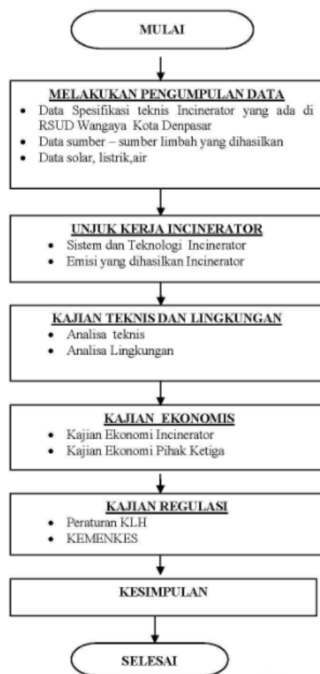
Gambar 5: Alur penelitian
