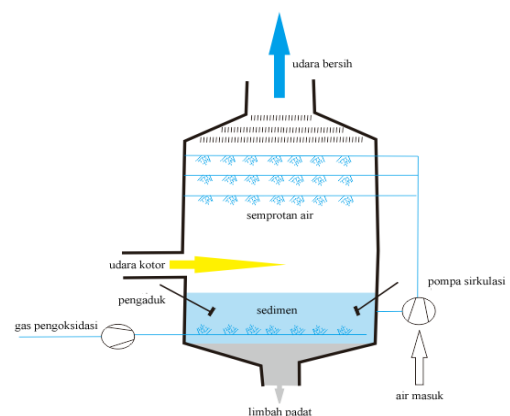
Gambar 3: Prinsip kerja Wet Scrubber
