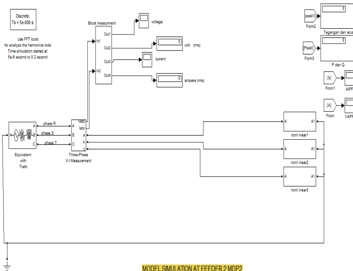
Gambar 2. Model Simulasi
