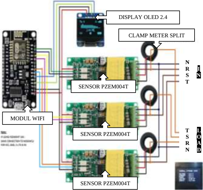
Gambar 4: Skematik Monitoring 3 Fase 3 Sensor PZEM004t Wirelles IoT
