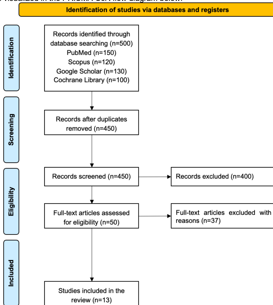
Figure 1. PRISMA Diagram
