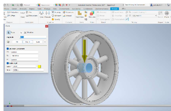
Gambar 5. Beban force
