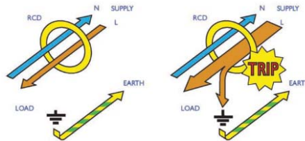
Gambar 2.3. Prinsip kerja RCD (residual Current Device)
