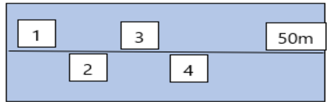
Gambar 3. Ilustrasi metode UPT (Giyanto, 2014)
