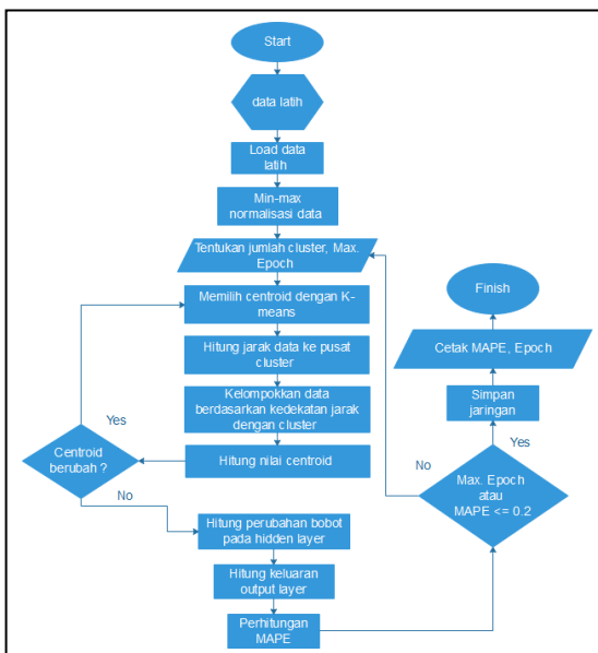
Gambar 1. Flowchart proses pelatihan
