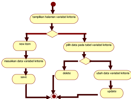
Activity Diagram Kelola Data Kriteria
