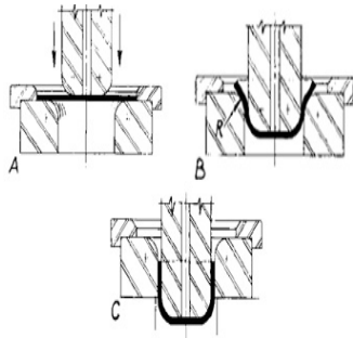
Gambar 1. Proses drawing
