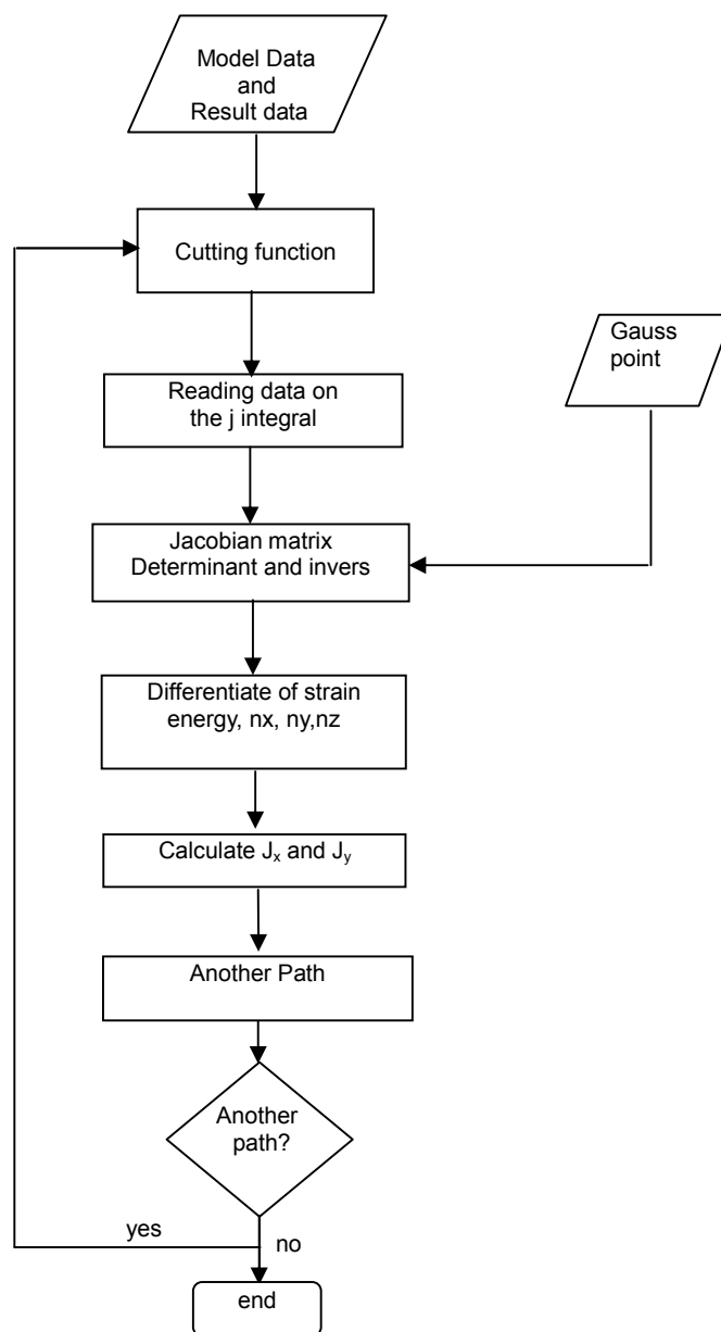
Gambar 2 Diagram alir prosedur analisa J-Integral
