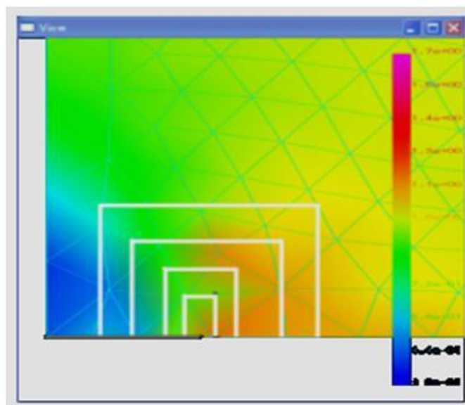
Gambar 5 J-integral path
