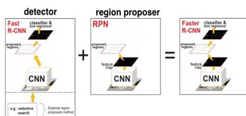
Fig. 4 R-CNN Faster Architecture
