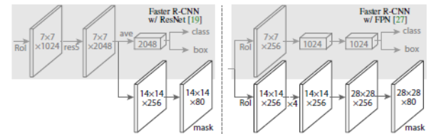
Fig. 5 Illustration of mask R-CNN
