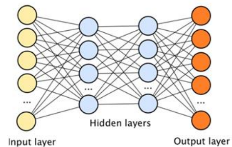
Fig. 2 Deep Learning
