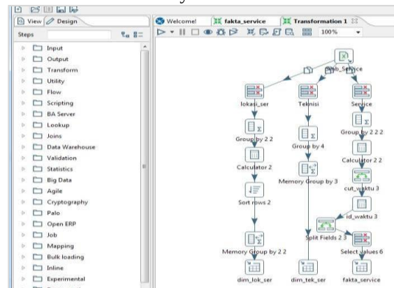
Fig 6. Processing Integration Sales Data
