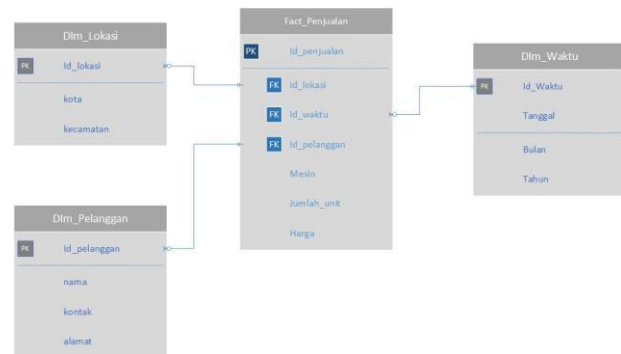
Fig 5. Schema Dimensional Sales Data
