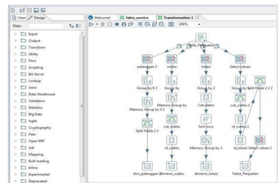
Fig 7. Processing Integration Service Data
