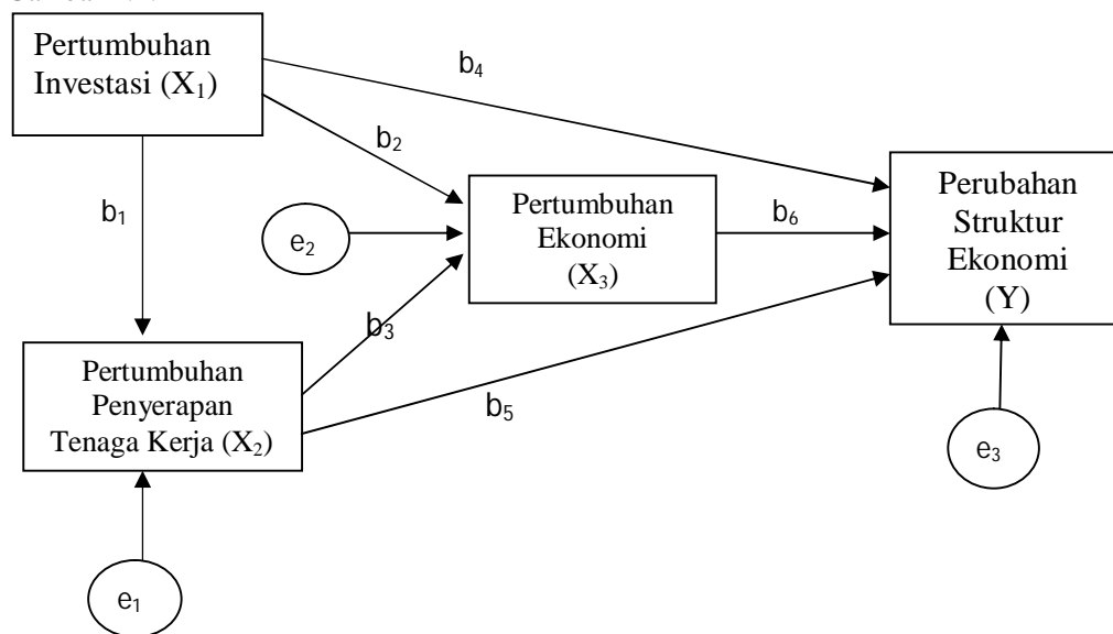
Gambar 4 Diagram Jalur Variabel Penelitian
