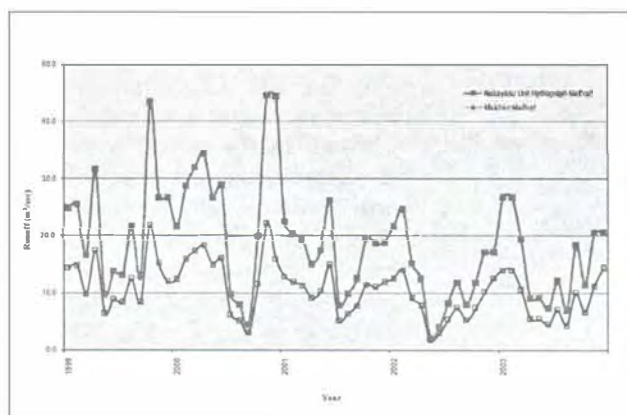
Figure 5 Monthly Average Runoff by Nakayasu Unit Hydrograph and Melchior Method from 1999 to 2003
