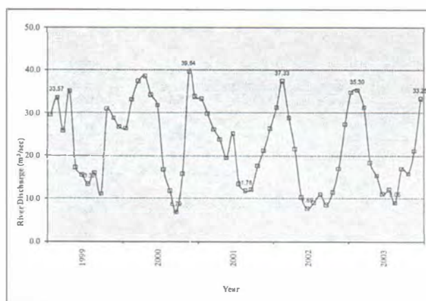
Figure 6 Monthly Average River Discharge from 1999 to 2003.
