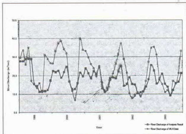
Figure 7 Monthly Average River Discharge from 1999 to 2003 (Nakayasu Unit Hydrograph Method and Water Level Recorder (WLR) Data)
