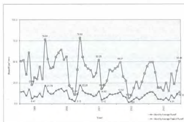
Figure 3 Monthly Average Runoff and Peak Runoff from 1999 to 2003 (Nakayasu Unit Hydrograph Method)
