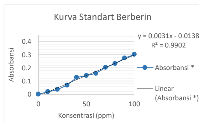
Gambar 1. Kurva Standart Berberin
