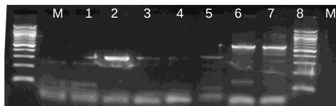
Fig. 2. Detection of CSVd (lanes 1-2), Potyvirus (lanes 3-4), ToCV (lanes 5-6) and CVB (lanes 7-8) by SDT-RT-PCR. Lane M: 100 bp DNA ladder (Fermentas)
