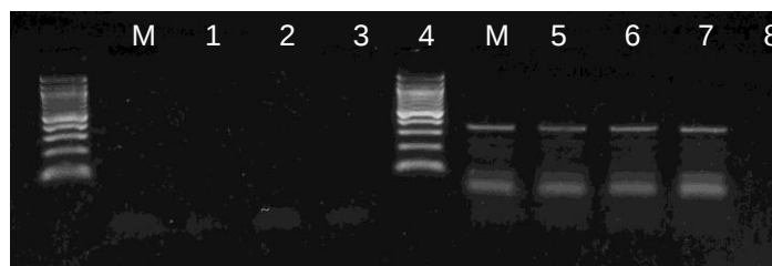
Fig. 4. Evaluation of dilution of crude sap prepared from Potyvirus infected leaves. Crude sap diluted 10^1 -, 10^2 -, 10^3 - or 10^4 -fold (lanes 5-8). Lane M: 100 bp DNA ladder (Fermentas)
