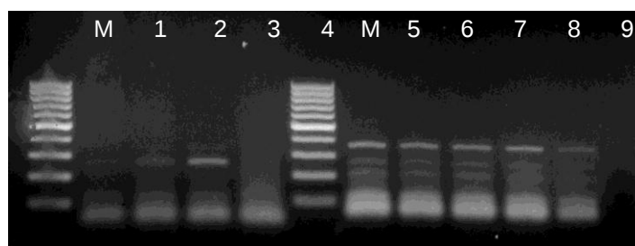
Fig. 3. Evaluation of dilution of crude sap prepared from infected leaves. Lanes 1-4; the crude sap prepared from CSVd infected leaves diluted 10^1 -, 10^2 -, 10^3 - or 10^4 -fold, respectively. Lanes 5-9; the crude sap prepared from ToCV infected leaves diluted 10^1 -, 10^2 -, 10^3 -, 10^4 - or 10^5 -fold, respectively. Lane M: 100 bp DNA ladder (Fermentas)
